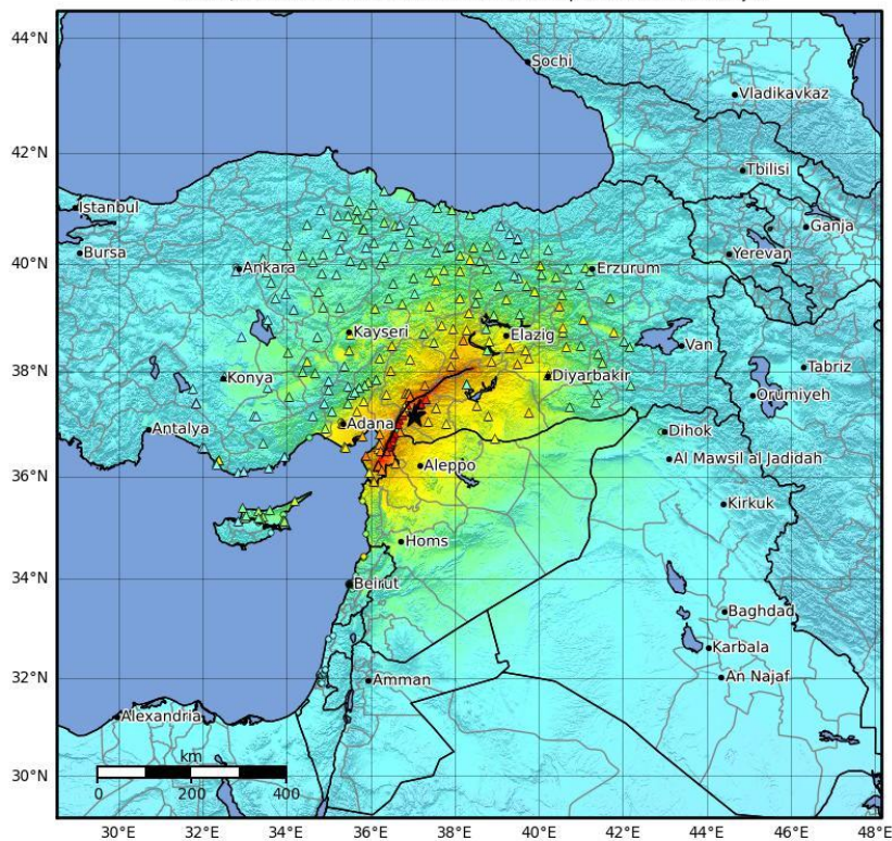
Macroseismic Intensity Map USGS ShakeMap: 26 km E of Nurdağı, Gaziantep, TR Feb 06, 2023 01:17:35 UTC M7.8 N37.17 E37.03 Depth: 17.9km ID:us6000jllz
